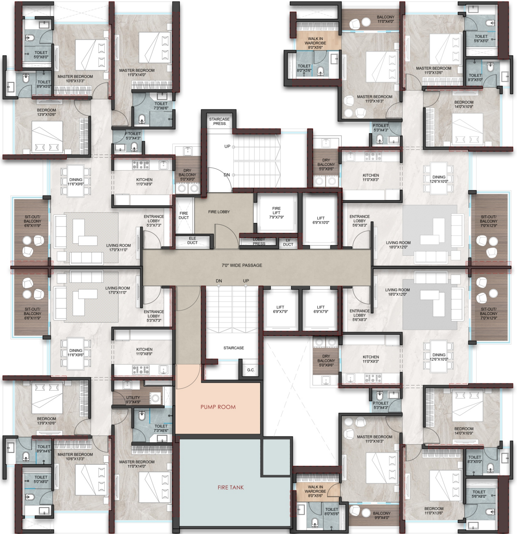
3BHK TYPE 03 CARPET=1276 SQ.FT
